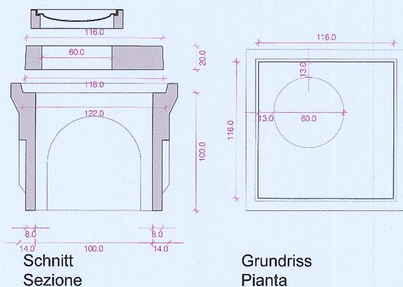
TRINKWASSERSCHACHT 100x100 POZZETTO ACQUA POTABILE 100x100 M 1 : 20
